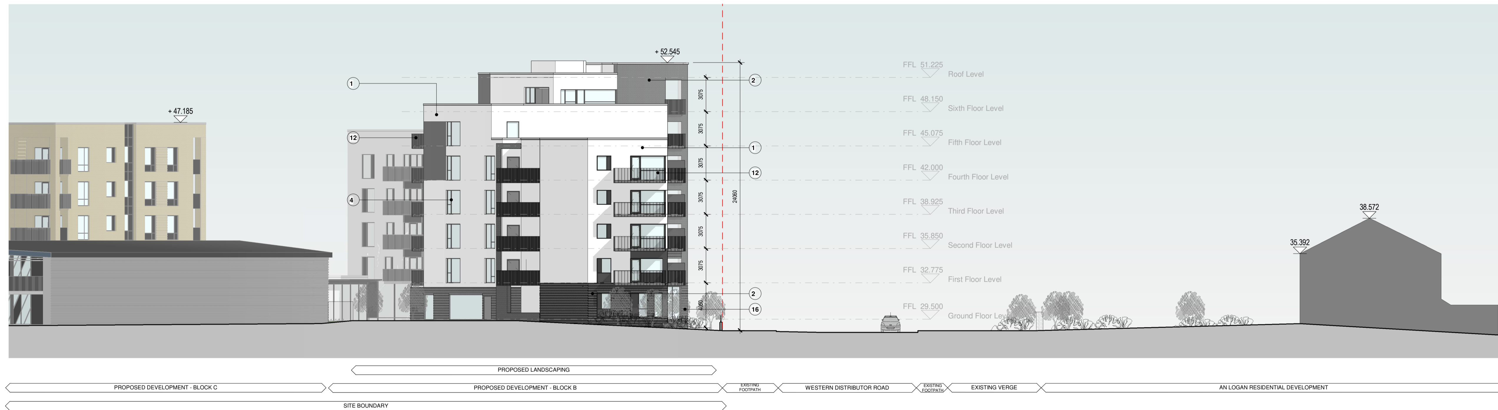
4 BLOCK B - WEST FACADE 1 : 200
